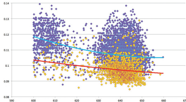
Griffin Open Systems (yellow) vs. N-Net (purple) ~10% Shift to Lower NO x on average
